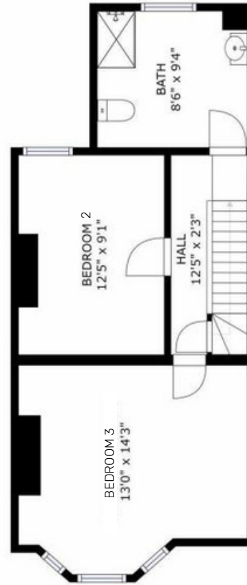
1st floor
